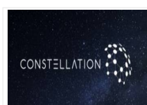
Constellation
